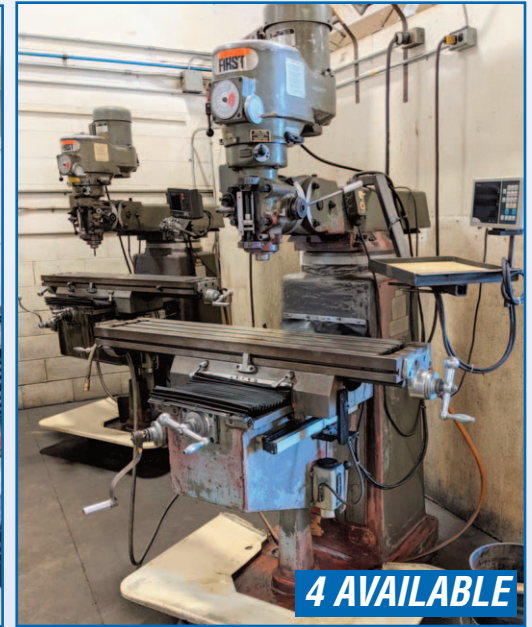
FIRST LC-185VS VERTICAL MILLING MACHINE
