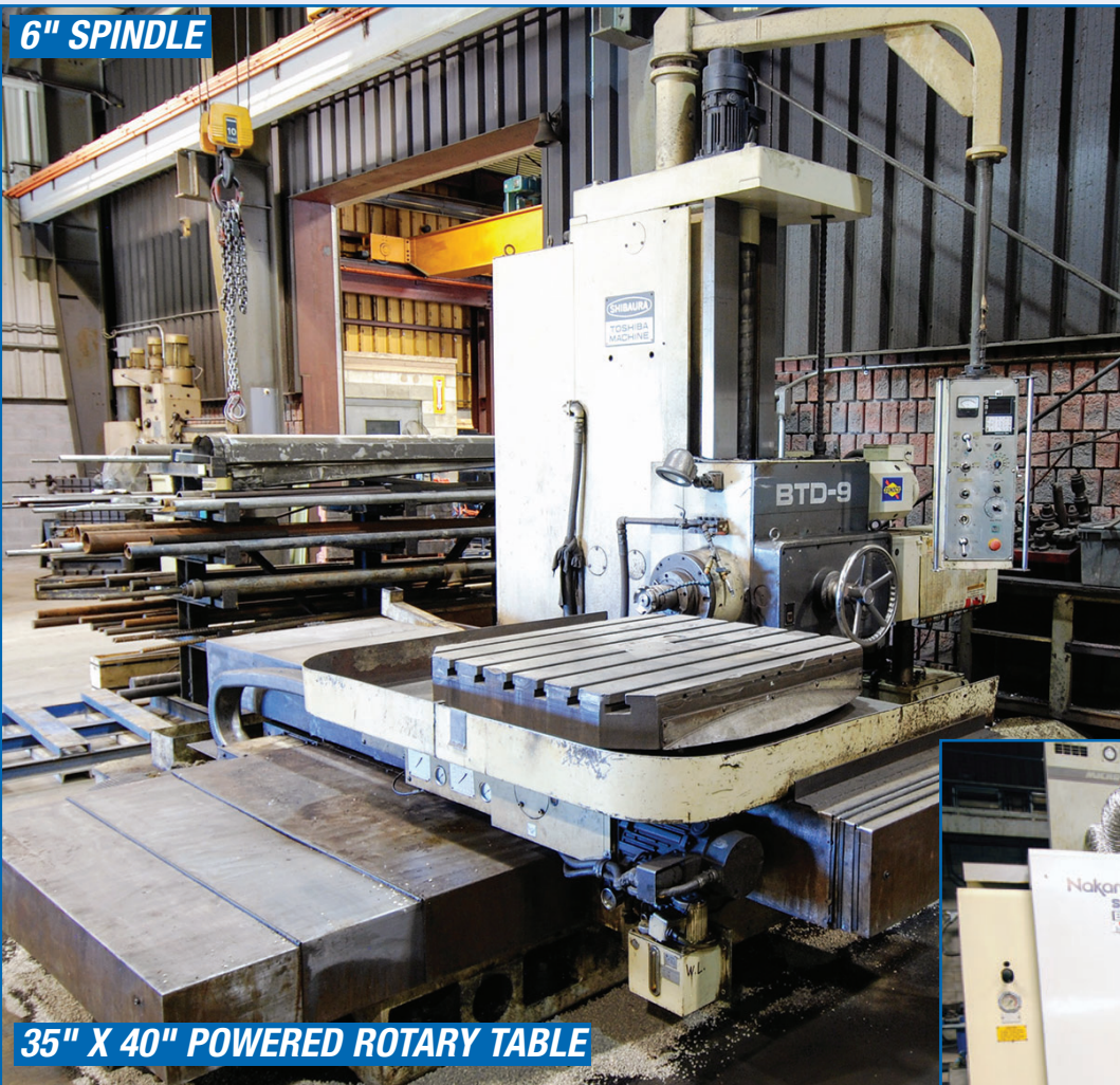
TOSHIBA SHIBAURA BTD-9 TABLE TYPE HORIZONTAL BORING MILL
