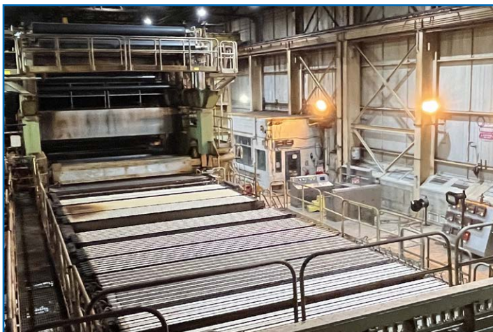
BLACK CLAWSON 178" Trim Paper Machine, 2200 Feet Per Minute, 480 Tons Per Day Max Output, 191" Slice Width, 195" Wire Cantilevered Fourdrinier, 50 Dryers (4 Sections), Super AUTOFLYTE 36" Reel, 187" Drum Face, MODULANT 186" Slitter Winder, B.T.H.B. 12"x191" Single Roll bunched Tube Headbox 9 PT Corrugated Medium Product, Travel from Right to Left s/n B-1160-1038
