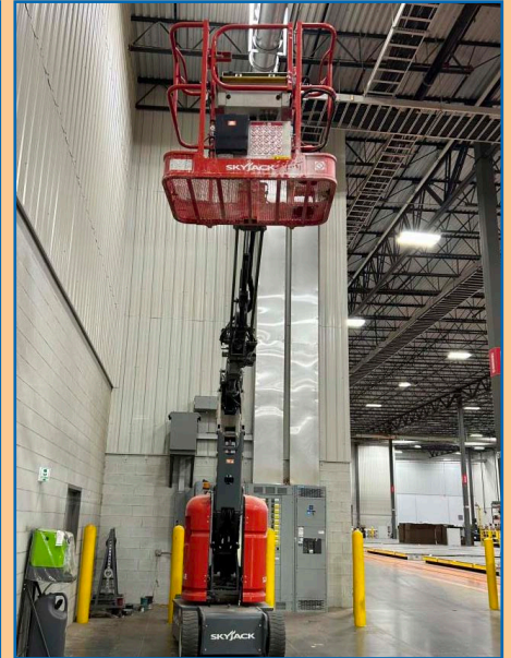
SKYJACK SJ30AJE BOOM LIFT
