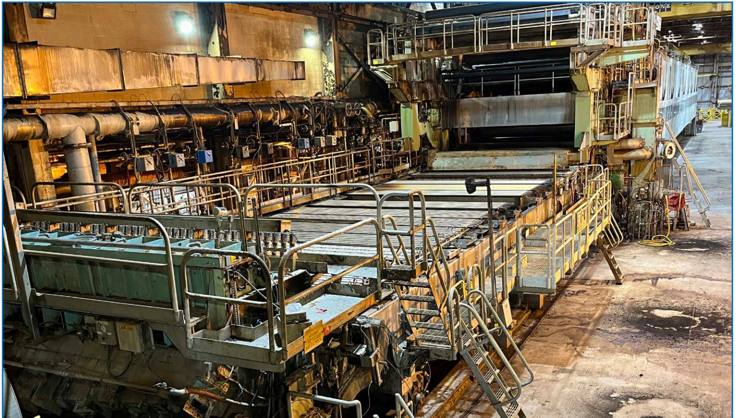
BLACK CLAWSON 178" Trim Paper Machine, 2200 Feet Per Minute, 480 Tons Per Day Max Output, 191" Slice Width, 195" Wire Cantilevered Fourdrinier, 50 Dryers (4 Sections), Super AUTOFLYTE 36" Reel, 187" Drum Face, MODULANT 186" Slitter Winder, B.T.H.B. 12"x191" Single Roll bunched Tube Headbox 9 PT Corrugated Medium Product, Travel from Right to Left s/n B-1160-1038
