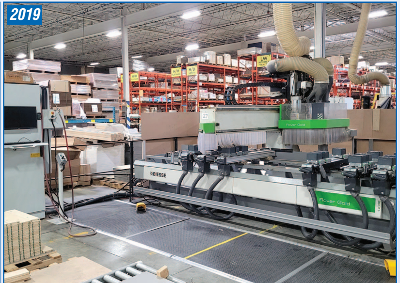
BIESSE ROVER GOLD 1232 COMPACT CNC MACHINING CENTER / ROUTER
