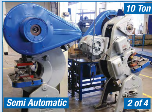
SWEENEY & BLOCKSIDE MODEL NO. 7, OBI PRESS
