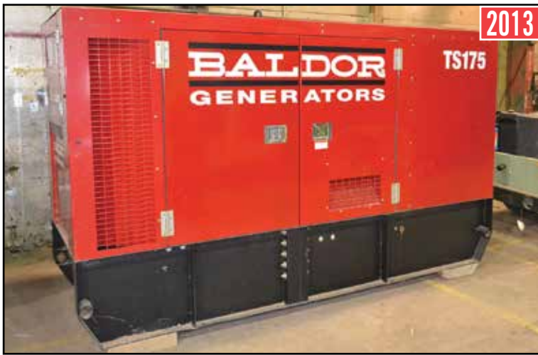
2013 BALDOR TS175 175 Kw Portable Skid-Mounted Diesel Generator
