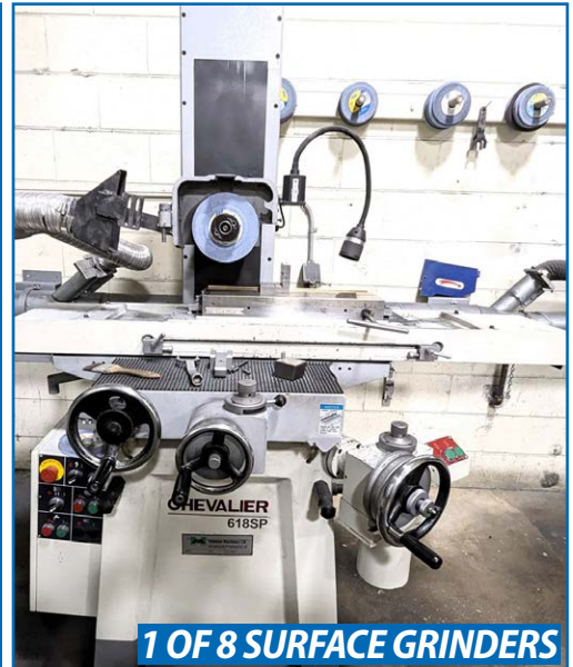
CHEVALIER 618SP SUPER PRECISION SURFACE GRINDER
