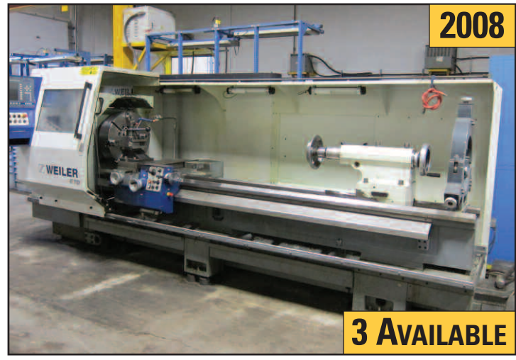
28.6" x 120" Weiler E70x3000 CNC Oilfield Engine Lathe
