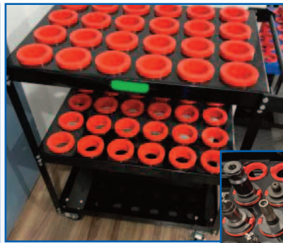
CAT 50 - BT 50, CNC TOOL CART
