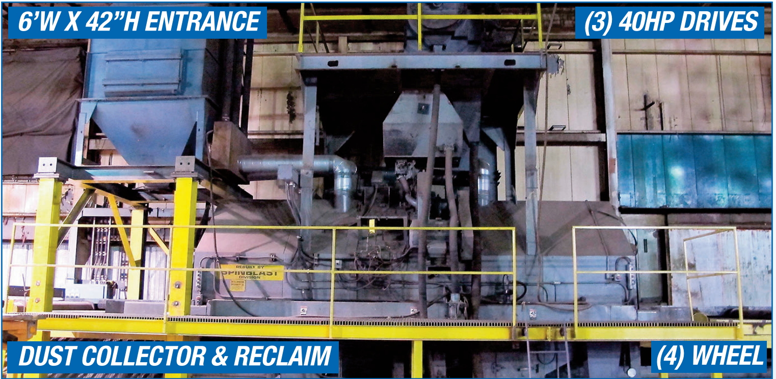
SHOTBLAST SYSTEM (REBUILT BY SPINBLAST)
