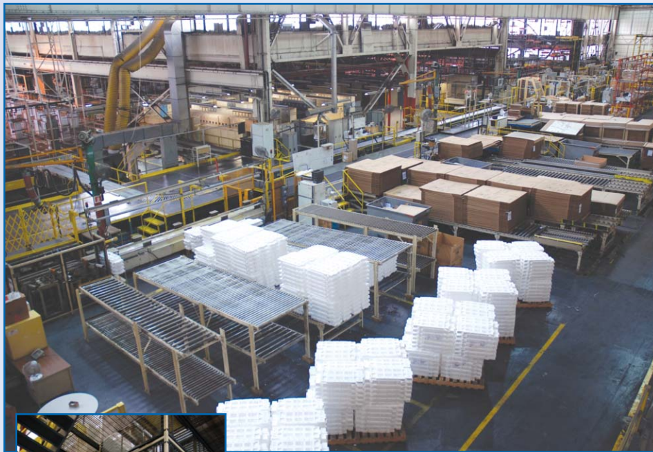
PARTIAL VIEW OF 5 PACKAGING LINES
