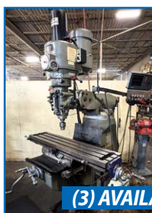
FIRST LC-1-1/2VS VERTICAL MILL
