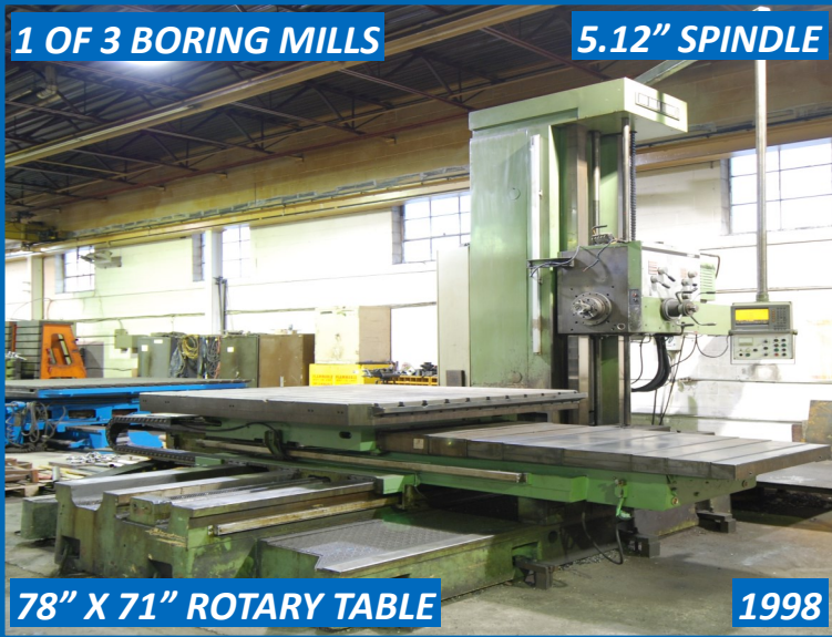
IVO LOLA RIBAR HBM5 HORIZONTAL BORING MILL
