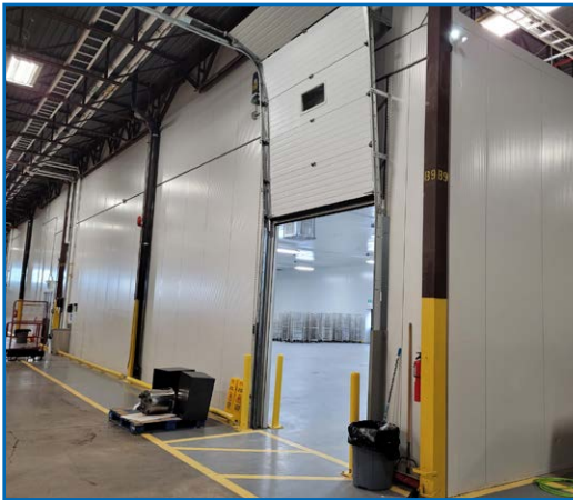
CLEAN ROOM INSULATED WALL PANEL STRUCTURE
