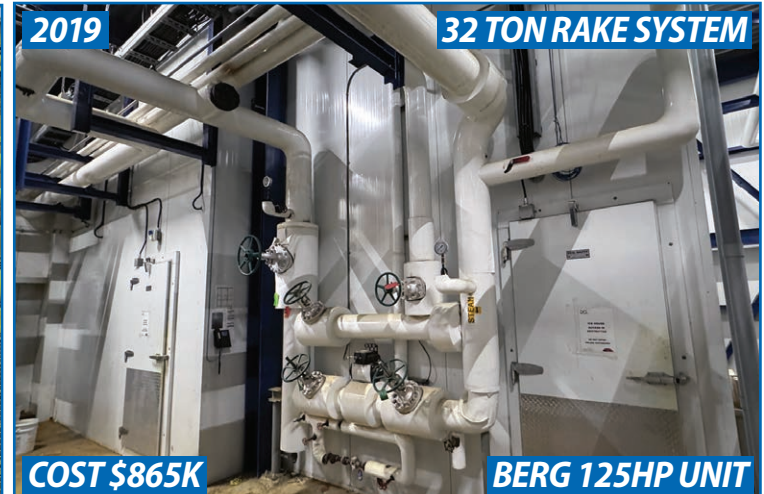
NORTHSTAR/BERG ICE MAKING PLANT
