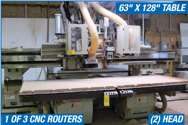
ANDERSON EXXACT DUO/MH CNC ROUTER
