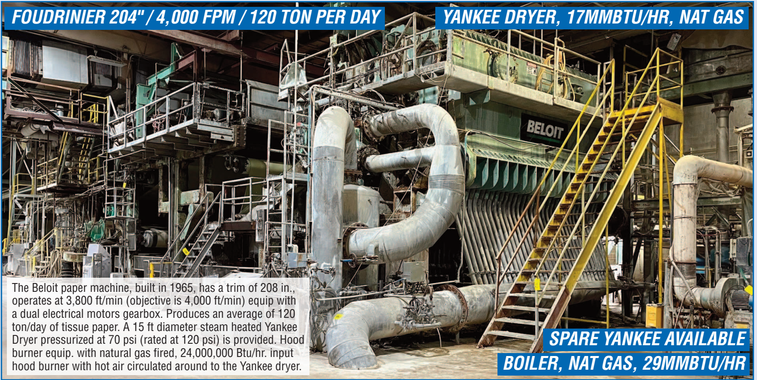
PARTIAL VIEW OF BELOIT PAPER MACHINE
